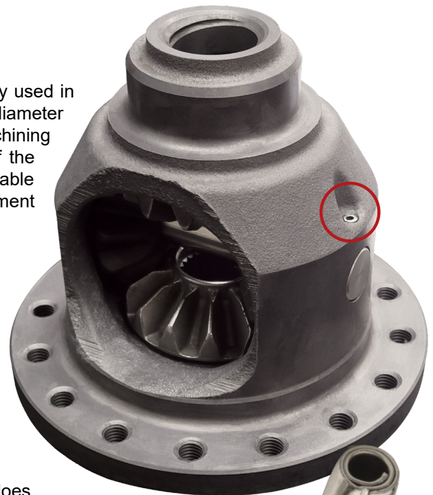
SPIROL Coiled Spring Pin retains a pinion shaft in a differential carrier assembly.
