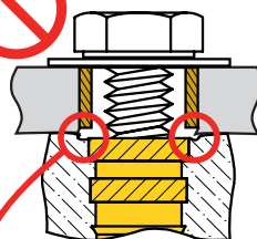
Plastic creep
