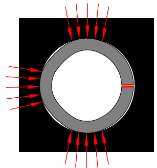
NON-DYNAMIC CONDITION Installed Slotted Pin showing the "Butted" condition making the pin unable to absorb dynamic loads
