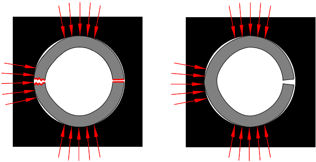
BREAK CONDITION Slotted Pin after fatigue failure at 180° from the gap
